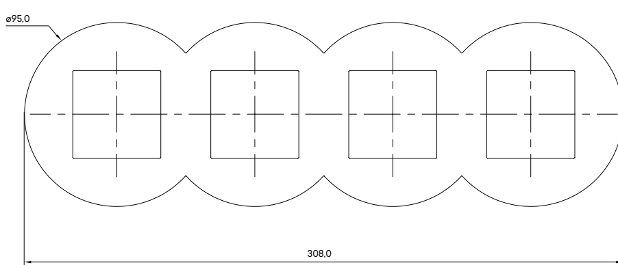
Ref. 43940 T - SV Four-Gang
