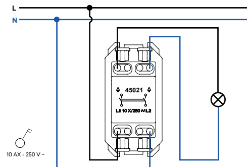
Interruptor Bipolar
