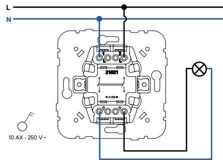
Interruptor Bipolar
